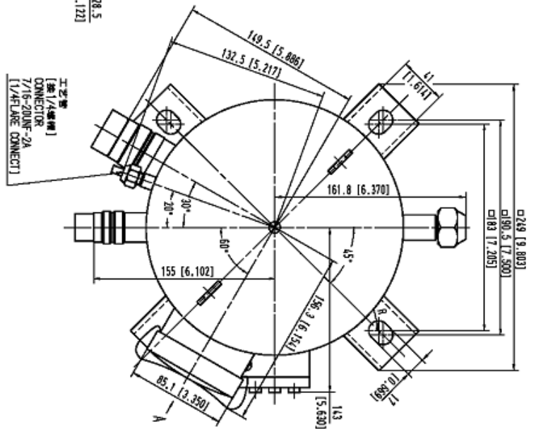
Part Code D-0110-DSC Name Compressor Outline Drawing
